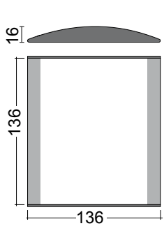
1 TÜRSCHILD 84200G
