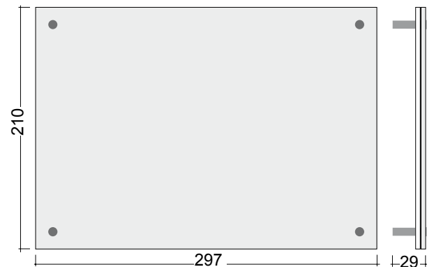
5 WANDSCHILD A4 QF 297 x 210 mm 84152G
